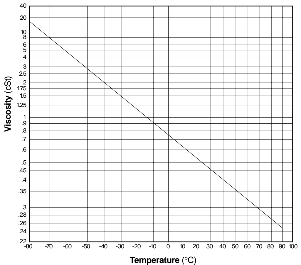
Fluorinert Liquid FC-84 Viscosity (cSt) vs. Temperature (°C)
